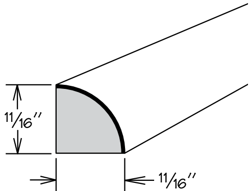
QUARTER ROUND
