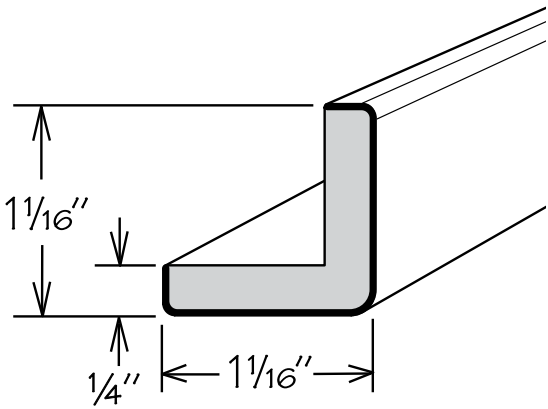
OUTSIDE CORNER
