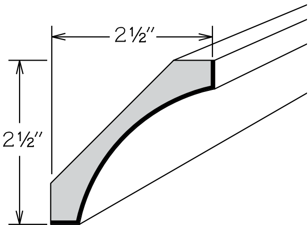
COVE CROWN
