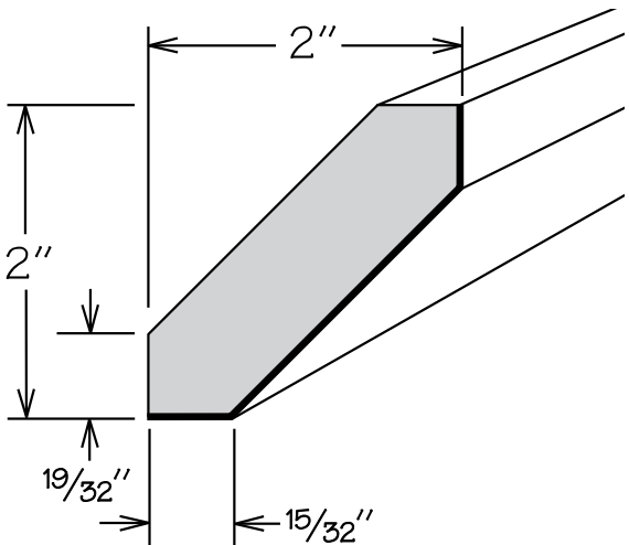
ANGLED CROWN
