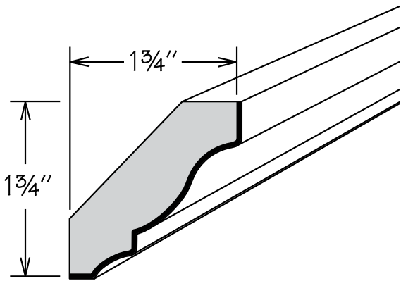
TRADITIONAL CROWN
