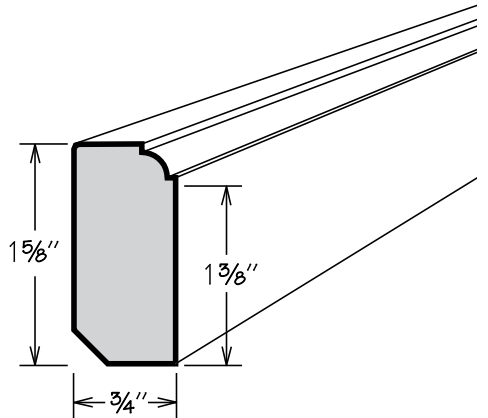
DECORATIVE TRIM
